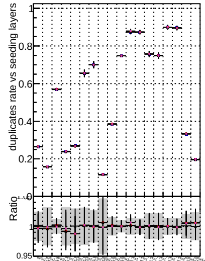
Ratio Legend: DOM, mktFit, T, Original, New Study v4, New Study v4p4
