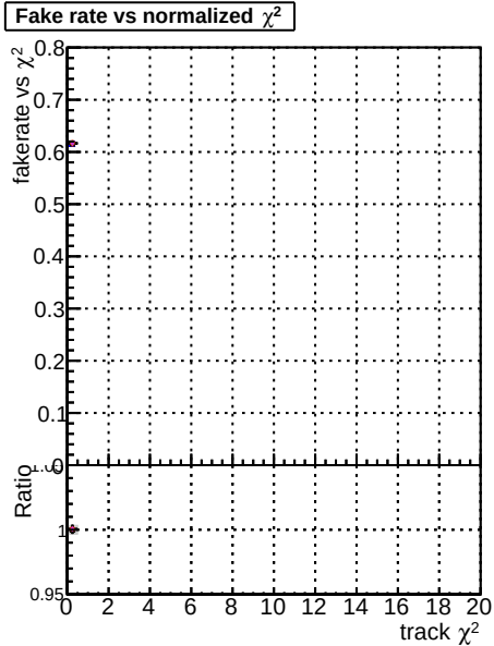
Fake rate vs. \chi^2 Legend: DOM, mktFit, T, Original, New Study v4, New Study v4p4
