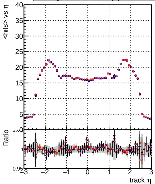
mean hits vs \eta Legend: DQM mkFit (blue), DQM mkFit (red), DQM mkFit (orange), DQM mkFit (purple), newStudy (black), newStudy4 (grey), newStudyhp4 (pink)
