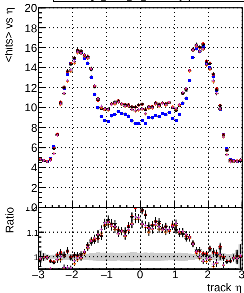
mean hits DOM mkFit TT original DOM mkFit TT newStudy DOM mkFit TT newStudy4 DOM mkFit TT newStudyh DOM mkFit TT newStudyhp4
