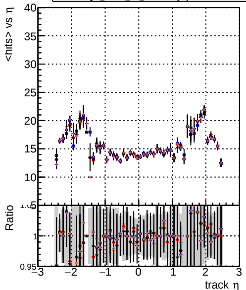
mean hit DOM mkFit TT original DOM mkFit TT newStudy DOM mkFit TT newStudy4 DOM mkFit TT newStudyh DOM mkFit TT newStudyhp4
