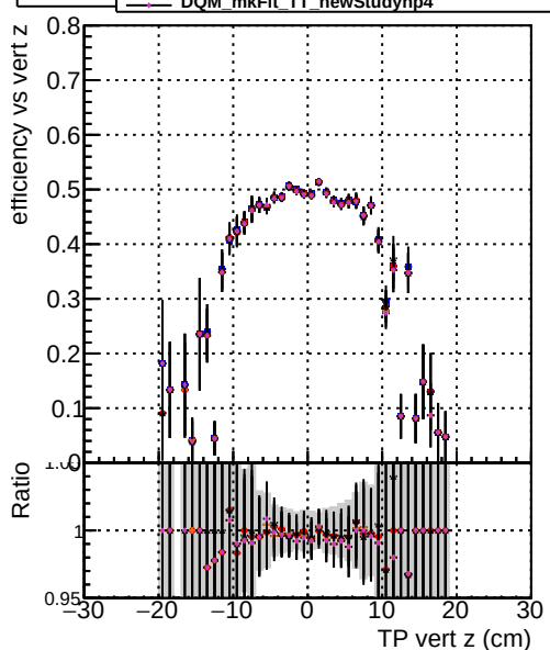
Effizienz Model Method Dataset ▲ DOM mkFit TT newStudyhp4 + DOM mkFit TT newStudyh DOM mkFit TT newStudyhp4
