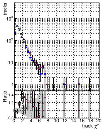
N of reco track vs. \chi^2 for Original, mFit, and new study v4
