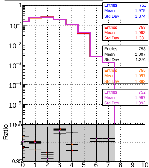
mean hit DOM mkFit TT original DOM mkFit TT newStudy DOM mkFit TT newStudy4 DOM mkFit TT newStudyhp4
