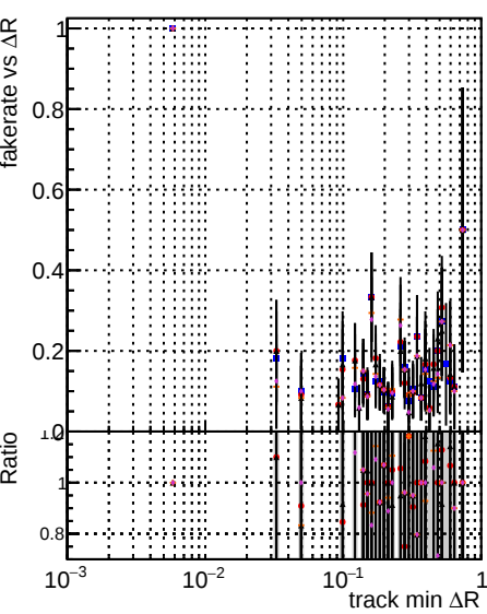
Fake rate vs \Delta R(\text{track, jet}) Legend: DOM (blue), mkFit (red), T-Original (green), newStudy (purple), newStudy4 (brown)
