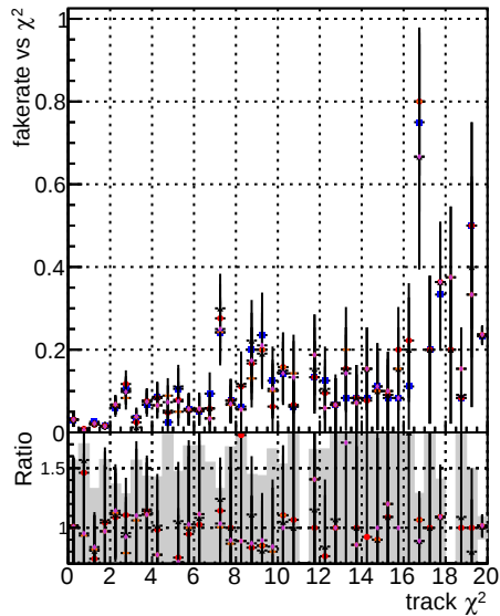
Fake rate vs. DOM mkFit DOM mkFit T T new study p4 new study p4
