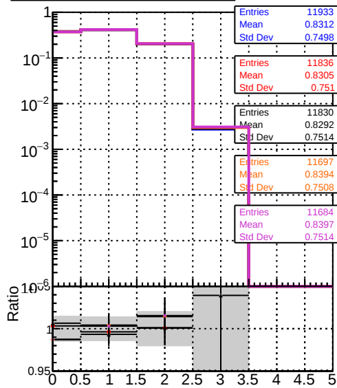
mean hit DOM mkFit original DOM mkFit newStudy DOM mkFit newStudyh4 DOM mkFit newStudyhp4
