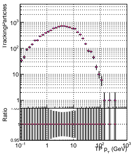
Legend for N of simulated tracks vs pT: Legend for N of associated tracks (simToReco) vs pT: — DQM mkFit original — DQM mkFit original — DQM mkFit newStudy — DQM mkFit newStudy — DQM mkFit newStudyhp4 — DQM mkFit newStudyhp4 — DQM mkFit newStudyh — DQM mkFit newStudyh — DQM mkFit newStudyhp4 — DQM mkFit newStudyhp4
