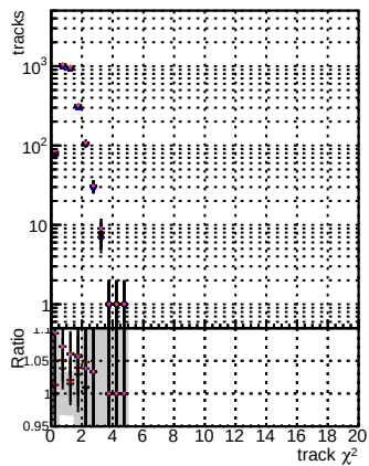
N of reco track vs. \chi^2 BOM mFit mFit mFit mFit mFit
