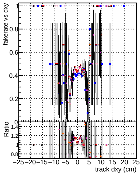
Legend for Fake rate vs dxy: DOM mktFit Toriginal DOM mktFit TnewStudy4 DOM mktFit TnewStudy4p4
