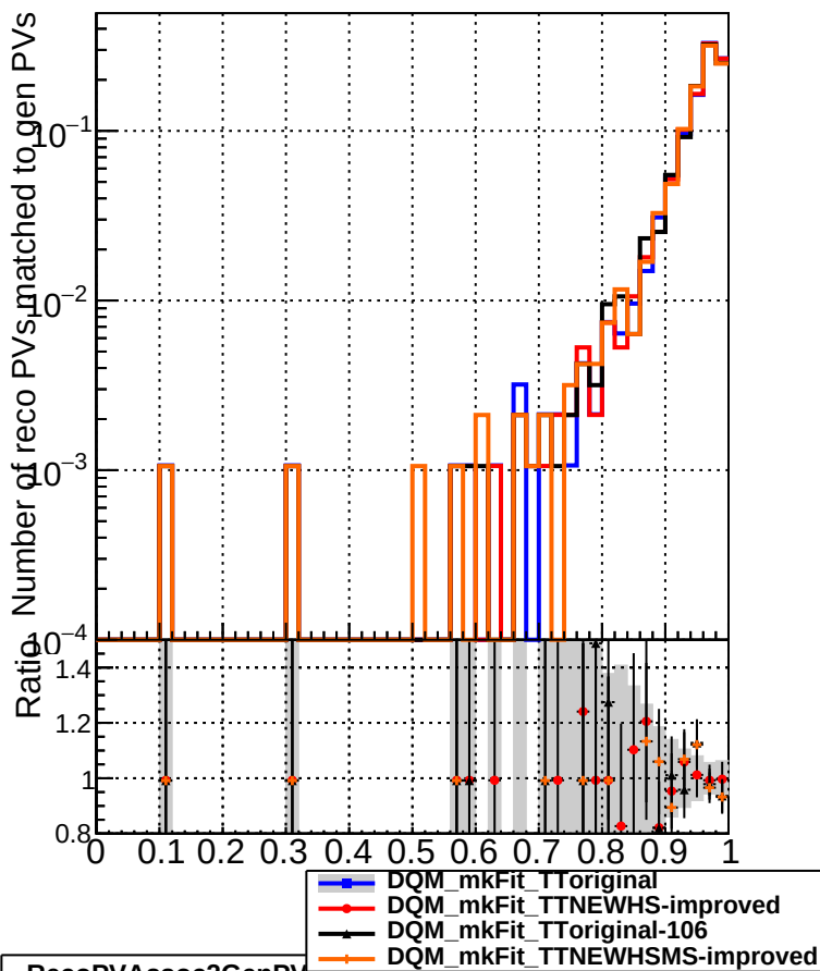
RecoPVAssoc2GenPVmatched_missing
