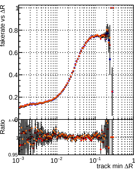
Fake rate vs \Delta R(\text{track, jet}) Legend: DOM (black), mktFit (blue), TR (red), TR-Improved (green), TR-Improved-100 (orange), TR-Improved-1000 (purple), TR-Improved-10000 (brown).
