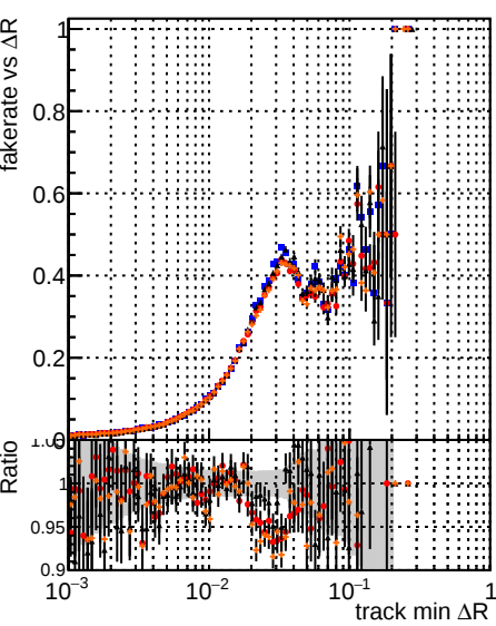
Fake rate vs \Delta R (track, jet) DOM mktFit T-Original T-Improved DOM mktFit NEWHS-100 NEWHS-100-improved DOM mktFit NEWHS-100-improved
