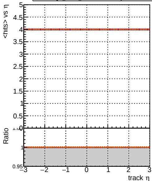
DQM_mkFit_TToriginal DQM_mkFit_TTNEWHs-improved DQM_mkFit_TToriginal-106 DQM_mkFit_TTNEWHsMS-improved
