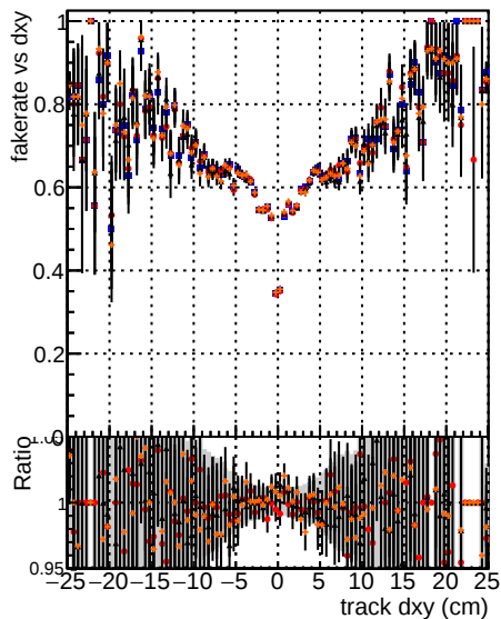
Legend for all plots: DSM mkFit DSM mkFit T-NEW improved DSM mkFit T-NEW improved DSM mkFit T-NEW improved
