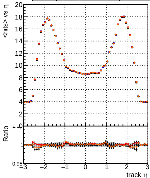
DQM_mkFit_TToriginal DQM_mkFit_TTNEWHS-improved DQM_mkFit_TToriginal-106 DQM_mkFit_TTNEWHSMS-improved mean hit
