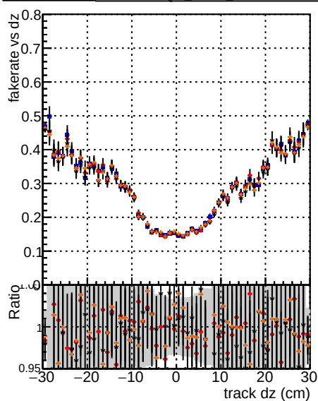
Fake rate vs dz Legend: DQM mktFit TTEV NEWHSM DQM mktFit TTEV improved DQM mktFit NEWHSM improved
