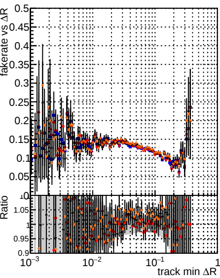
Fake rate vs \Delta R (track, jet) Legend: DOM (black) mktFit (blue) TR (red) Original (green) NEWHS-improved (orange) NEWHS-improved (orange) NEWHS-improved (orange)
