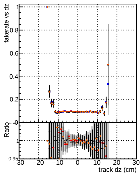
Fake rate vs dz Legend: DOM mkrFit TFWAS-improved DOM mkrFit+TFWAS-improved NEWHSM-improved
