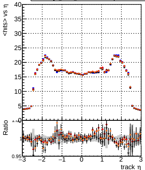
DQM_mkFit_TToriginal DQM_mkFit_TTNEWHMS-improved DQM_mkFit_TToriginal-106 DQM_mkFit_TTNEWHMSMS-improved mean hits
