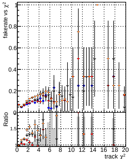
Fake rate vs. \chi^2 Legend: DQM mktFit TT-neural-improved DQM mktFit TT-neural-improved-log
