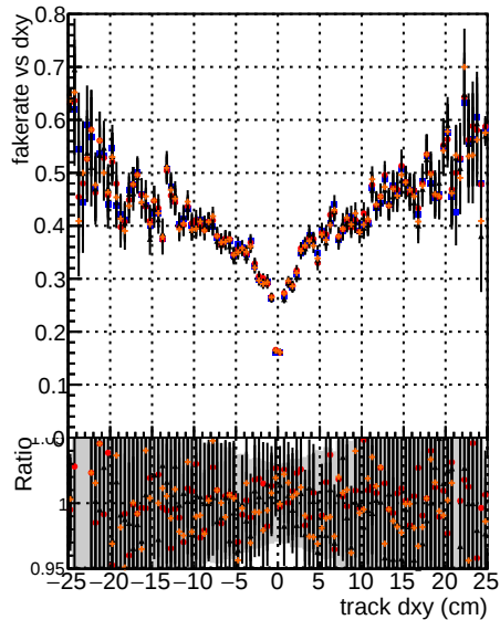
Legend for Fake rate vs dxy and other plots: DQM mkt fit T Toriginal Tnew Tnew-improved TnewHSM-improved
