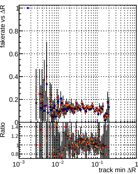
Fake rate vs \Delta R(\text{track, jet}) Legend: DOM mktFit Original DOM mktFit NEWHS-improved DOM mktFit NEWHS-improved
