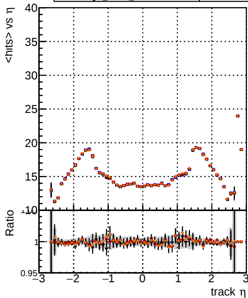
mean hits DQM_mkFit_TToriginal DQM_mkFit_TTNEWHMS-improved DQM_mkFit_TToriginal-106 DQM_mkFit_TTNEWHMS-improved
