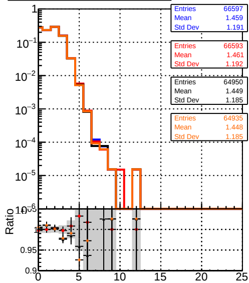
mean hits DQM_mkFit_TToriginal DQM_mkFit_TTNEWHMS-improved DQM_mkFit_TToriginal-106 DQM_mkFit_TTNEWHMS-improved
