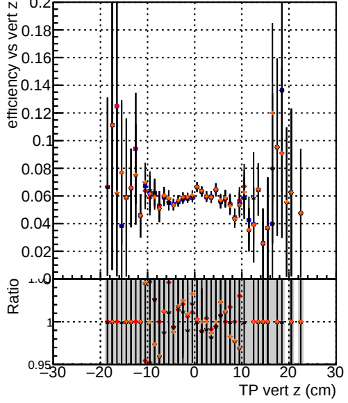
Efficiency vs. TP vert z (cm) Legend: - \bullet DQM_mkFit_TToriginal - \circ DQM_mkFit_TTNEWSMS-improved - \star DQM_mkFit_TToriginal-106 - \times DQM_mkFit_TTNEWSMS-improved
