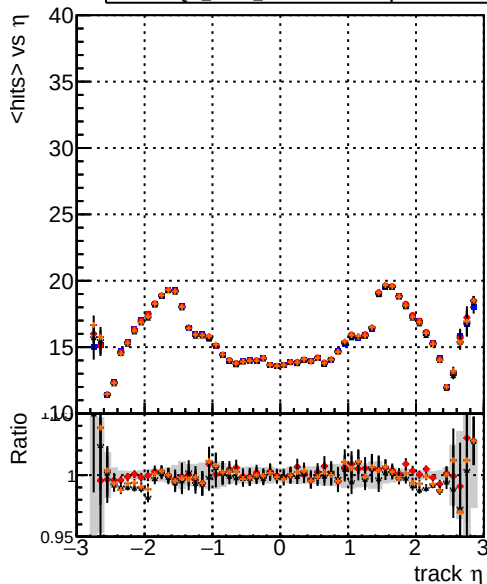
mean hits vs \eta DQM_mkFit_TToriginal DQM_mkFit_TTNEWHs-improved DQM_mkFit_TToriginal-106 DQM_mkFit_TTNEWHsMS-improved
