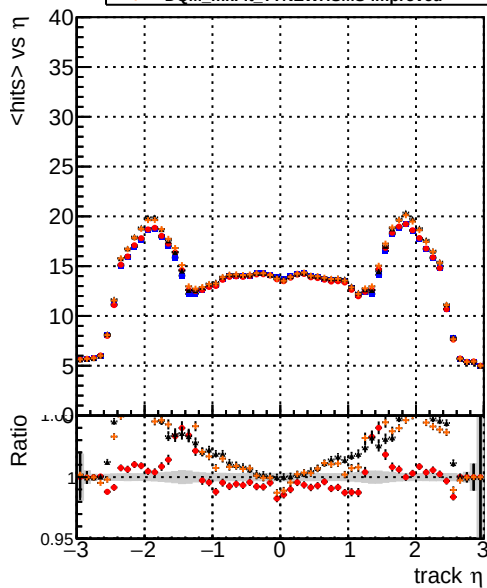
mean hits — DQM_mkFit_TToriginal — DQM_mkFit_TTNEWHs-improved — DQM_mkFit_TToriginal-106 — DQM_mkFit_TTNEWHsMS-improved
