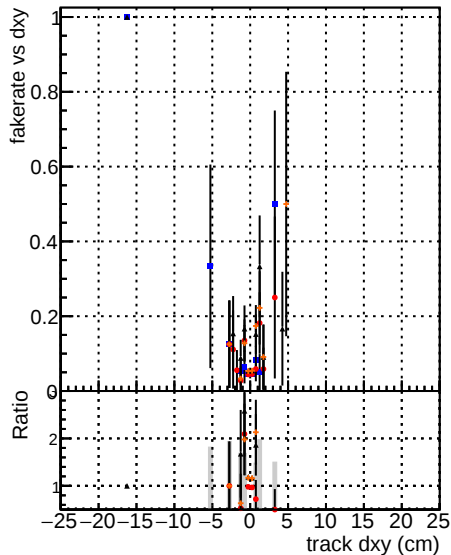
Legend for Fake rate vs dxy: DSM mktFit TToriginal DSM mktFit TTnewS-improved DSM mktFit TTnewS-improved
