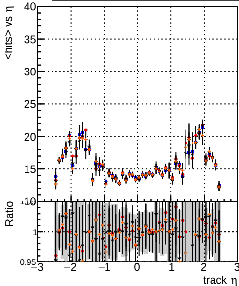
Legend: DQM_mkFit_TToriginal (blue), DQM_mkFit_TTNEWHMS-improved (red), DQM_mkFit_TToriginal-106 (black), DQM_mkFit_TTNEWHMSMS-improved (orange) mean hits
