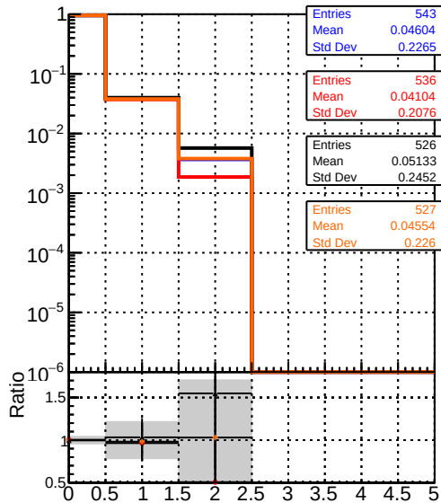
DQM_mkFit_TToriginal DQM_mkFit_TTNEWHs-improved DQM_mkFit_TToriginal-106 DQM_mkFit_TTNEWHsMS-improved
