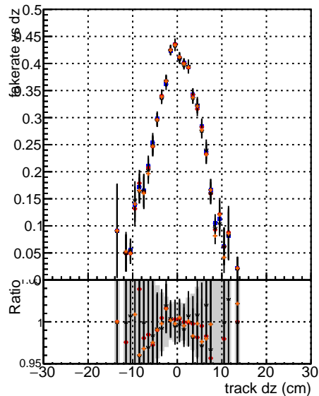
Fake rate vs dz ● BCG mkFit TToriginal ○ BCG mkFit TTnewSMS-improved ● BCG mkFit TTnewSMS-improved ○ BCG mkFit TTnewSMS-improved
