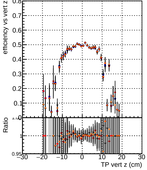
Efficiency vs. sim PV z —●— DQM_mkFit_TToriginal —●— DQM_mkFit_TTNEWHWS-improved —●— DQM_mkFit_TToriginal-106 —●— DQM_mkFit_TTNEWHSMS-improved
