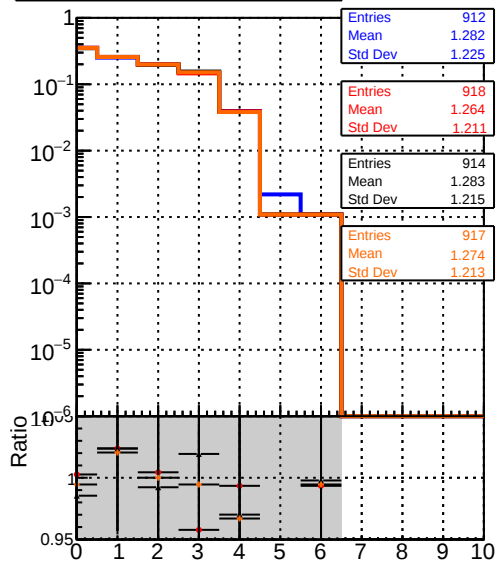
mean hit DQM_mkFit_TToriginal DQM_mkFit_TTNEWHMS-improved DQM_mkFit_TToriginal-106 DQM_mkFit_TTNEWHMSMS-improved
