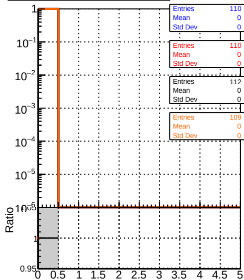
mean hit DQM_mkFit_TToriginal DQM_mkFit_TTNEWHMS-improved DQM_mkFit_TToriginal-106 DQM_mkFit_TTNEWHMSMS-improved
