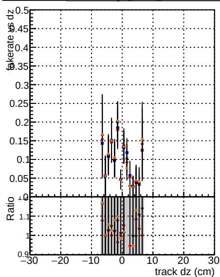
Fake rate vs dz Legend: DOM mktFit TToriginal DOM mktFit TTnewSMS-improved DOM mktFit TTnewSMS-improved
