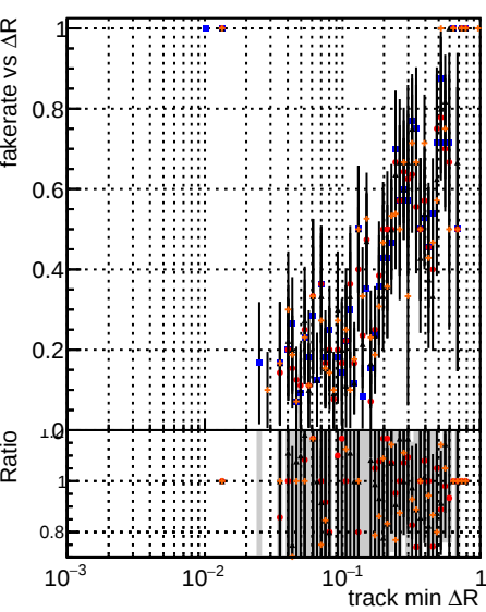
Fake rate vs \Delta R (track, jet) Legend: DOM mktFit T-Original T-improved NEWHS-100 NEWHS-improved
