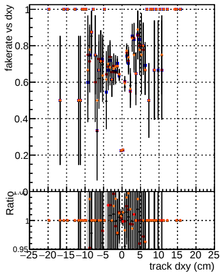
Legend for Fake rate vs dxy: DOM mkrFit DOM mkrFit TFWAS-improved DOM mkrFit NEWHSM-improved
