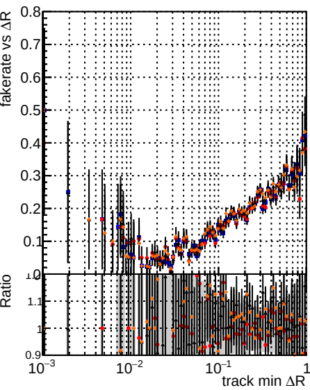
Fake rate vs \Delta R(\text{track, jet}) Legend: Original (black line) mktFit (blue line) NEWHS-improved (red line) NEWHS-improved (red line) NEWHS-improved (red line)
