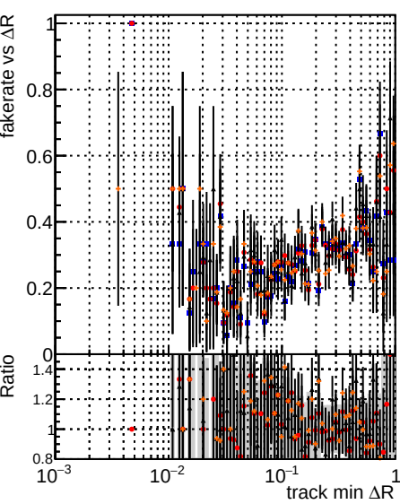
Fake rate vs \Delta R(\text{track, jet}) Legend: DOM mktFit T-Original DOM mktFit T-Original-improved DOM mktFit T-Original-improved DOM mktFit T-Original-improved
