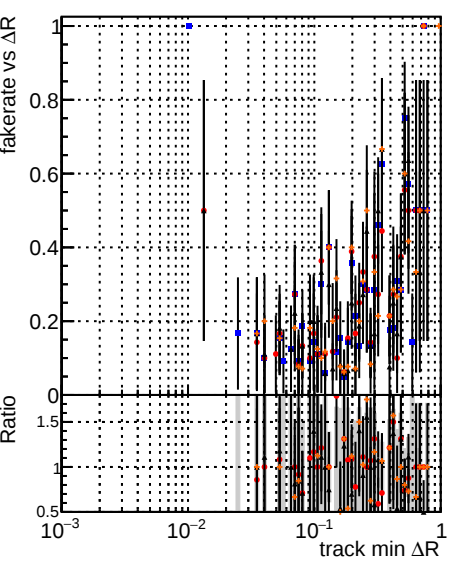
Fake rate vs \Delta R(\text{track, jet}) Legend: DOM mktFit T-Original T-Improved NEWHS-100 NEWHS-100-improved
