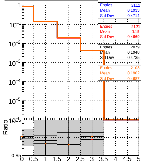
mean hit DQM_mkFit_TToriginal DQM_mkFit_TTNEWHMS-improved DQM_mkFit_TToriginal-106 DQM_mkFit_TTNEWHSMS-improved
