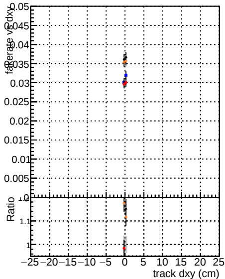
Legend for Fake rate vs dxy, Duplicates Rate vs Dxy, and Pileup rate vs dxy: DOM mktFit TToriginal DOM mktFit TTnewSMS-improved DOM mktFit TTnewSMS-improved
