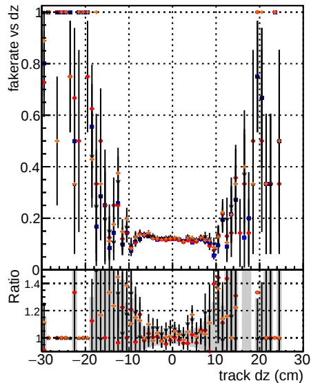
DOM mkrFit TTEVA TTEVA-improved DOM mkrFit TTEVA-improved NEWHSM-improved
