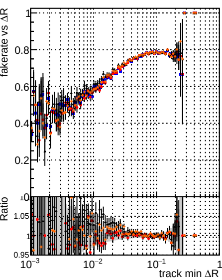
Fake rate vs \Delta R(\text{track, jet}) Legend: DOM mktfit TR original DOM mktfit TR WHS-improved DOM mktfit TR WHS-improved
