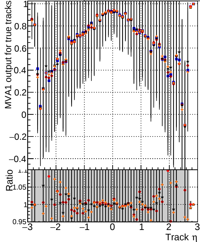
MVA1 of associated tracks (recoToSim) vs. track \eta Legend: ■ DQM_mkFit_TToriginal ■ DQM_mkFit_TTNEWHs-improved ■ DQM_mkFit_TToriginal-106 ■ DQM_mkFit_TTNEWHsMS-improved
