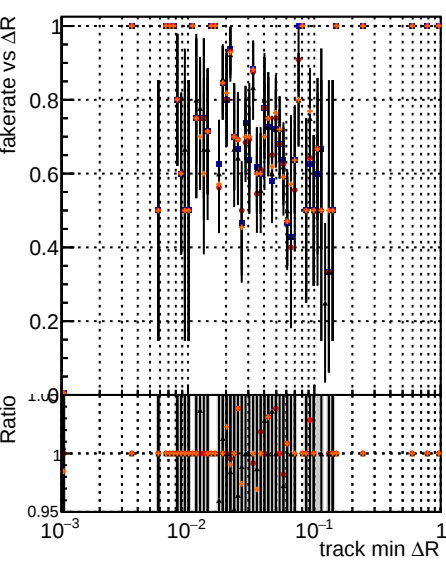
Fake rate vs \Delta R(\text{track, jet}) Legend: DOM mktFit T-Original DOM mktFit NEWHS-improved DOM mktFit NEWHS-improved
