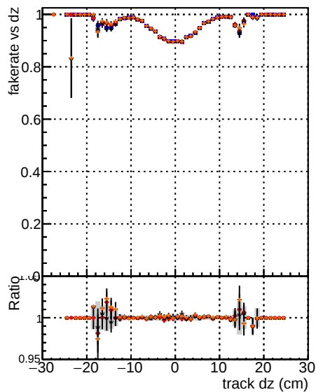
Legend: — BSM mktFit TToriginal — BSM mktFit TTnewS-improved — BSM mktFit TTnewS-improved
